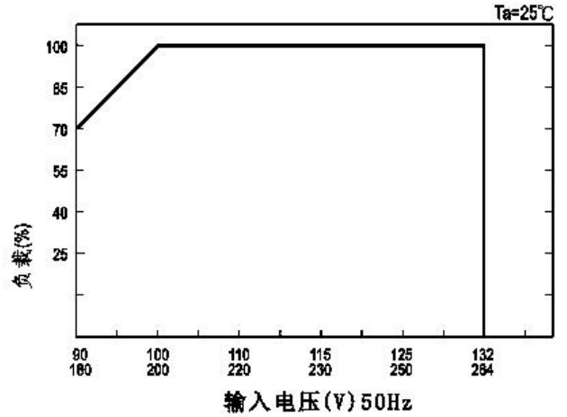
Static Characteristics:
